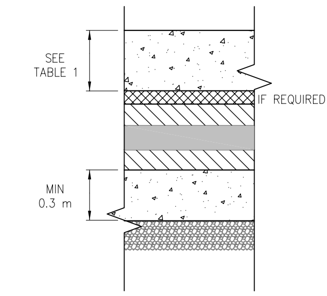
5 FLOOR & APPROACH WCF-1 NOT TO SCALE
