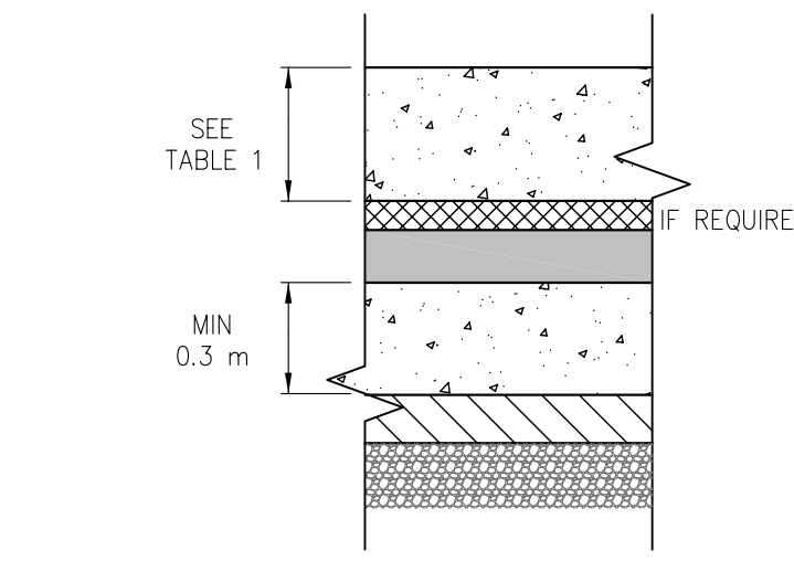
3 FLOOR & APPROACH WCF-1 NOT TO SCALE
