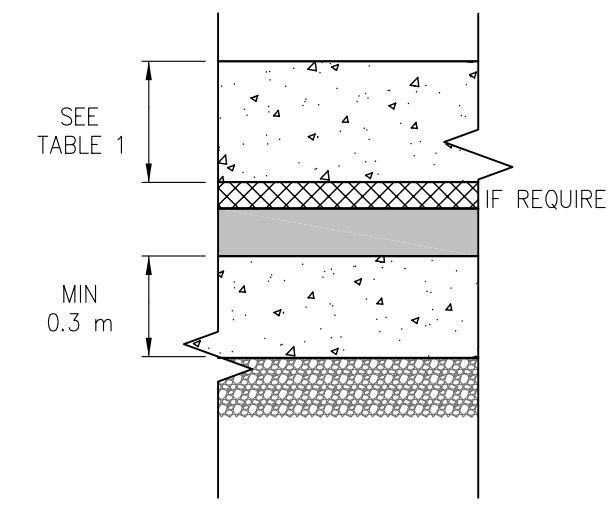
1 FLOOR & APPROACH WCF-1 NOT TO SCALE
