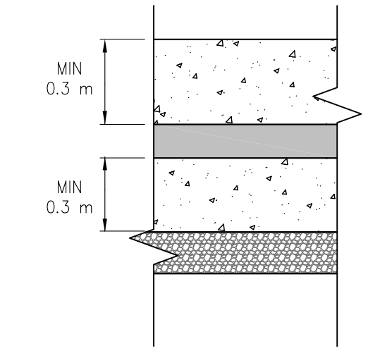
2 BERM WCF-1 NOT TO SCALE
