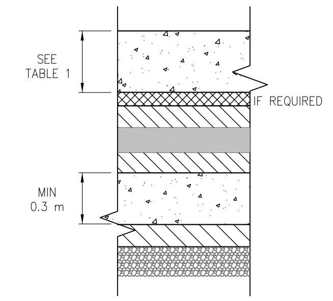
7 FLOOR & APPROACH WCF-1 NOT TO SCALE
