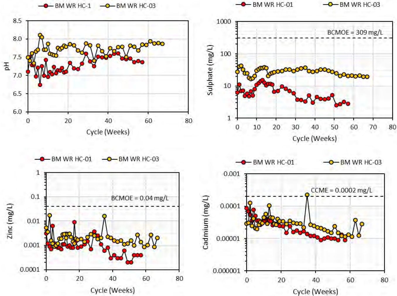
Figure 5-4: pH, Sulphate, Zinc and Cadmium Trends within the Bermingham N-AML Waste Rock Humidity Cells
