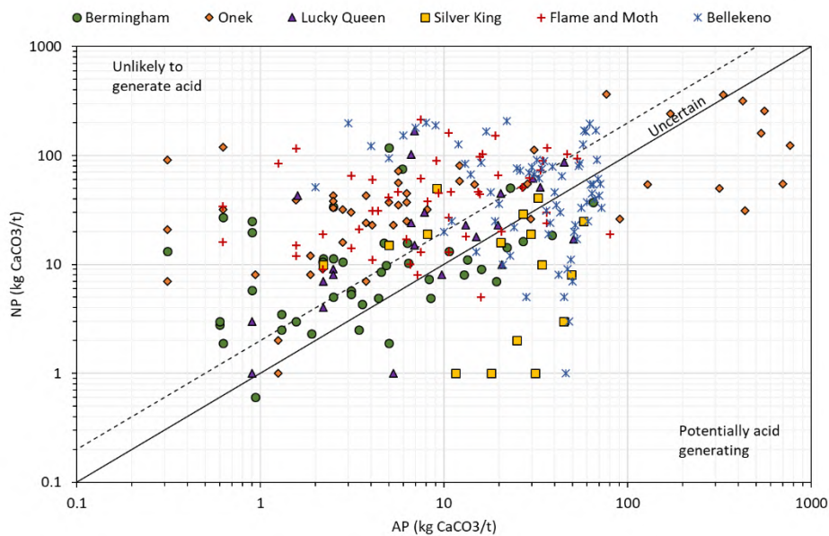
Figure 4-2: Variability in NP and AP of Waste Rock Samples from KHSD Deposits
