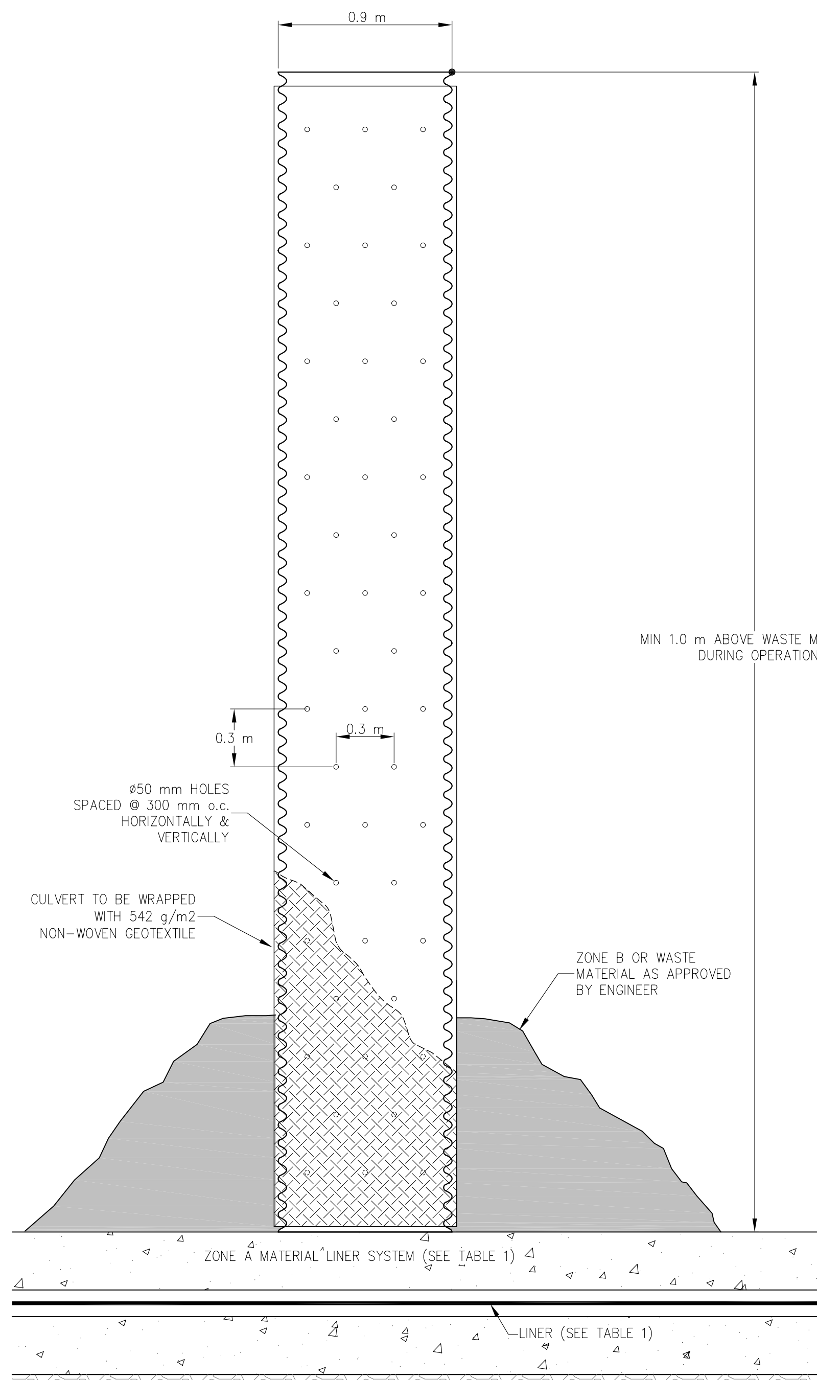
DETAIL 1 – VERTICAL CULVERT SCALE: 1 : 20
