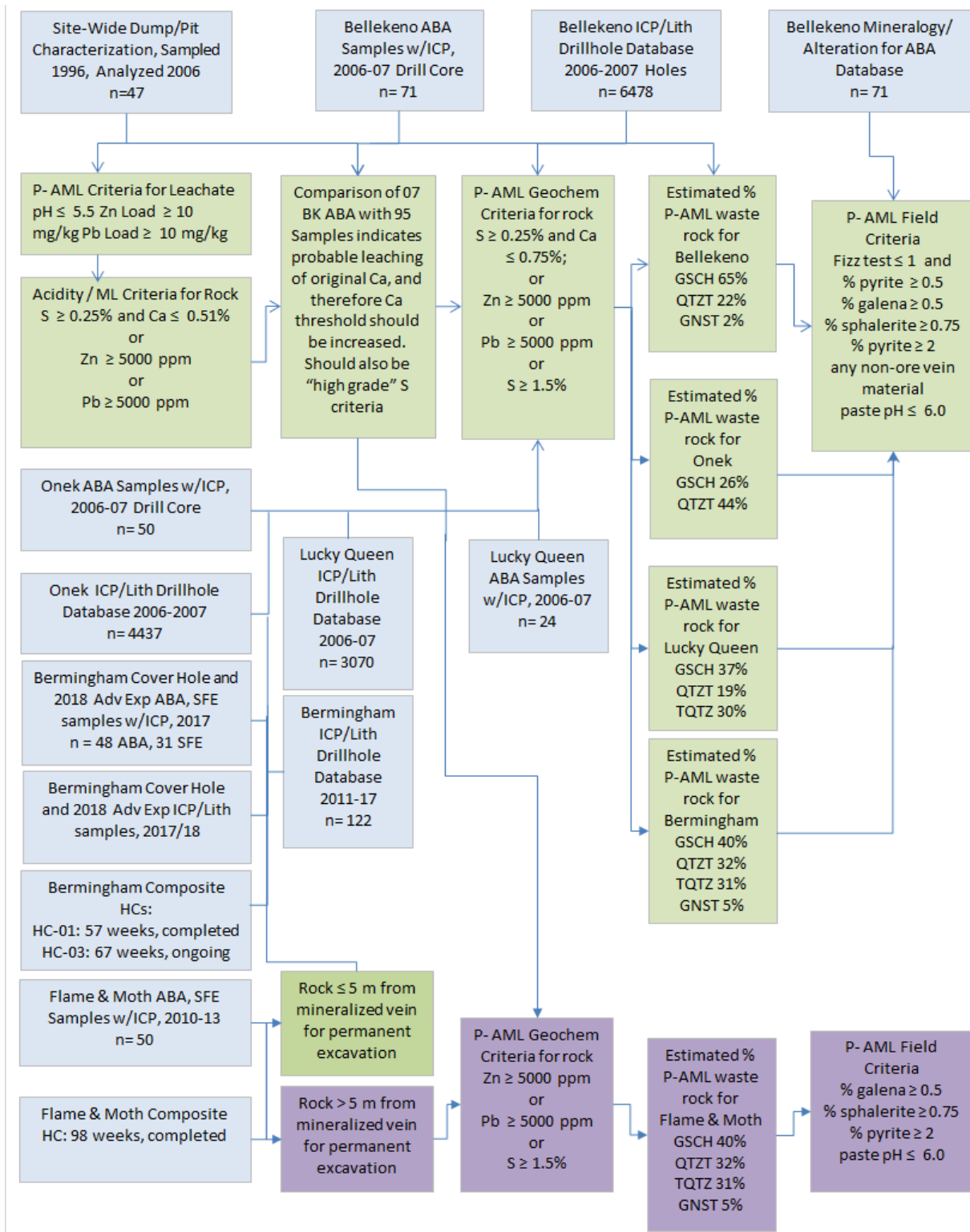
Figure 3-1: Keno Hill Development Waste Rock Characterization Studies – Components and Key Results
