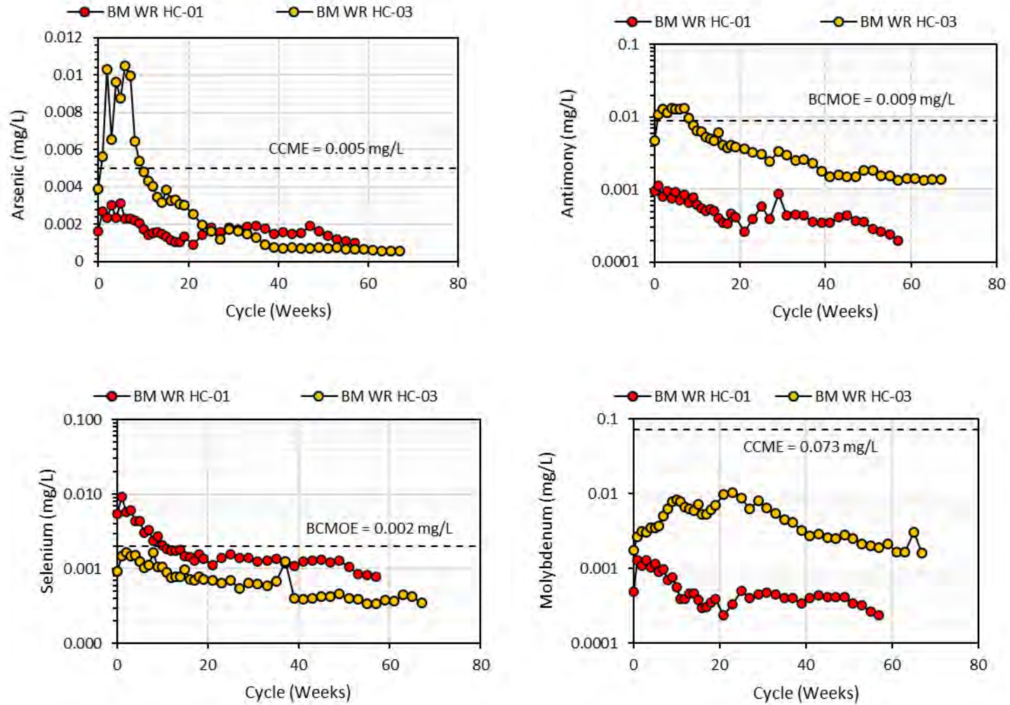
Figure 5-6: Arsenic, Antimony Selenium and Molybdenum Trends within the Birmingham N-AML Waste Rock Humidity Cells
