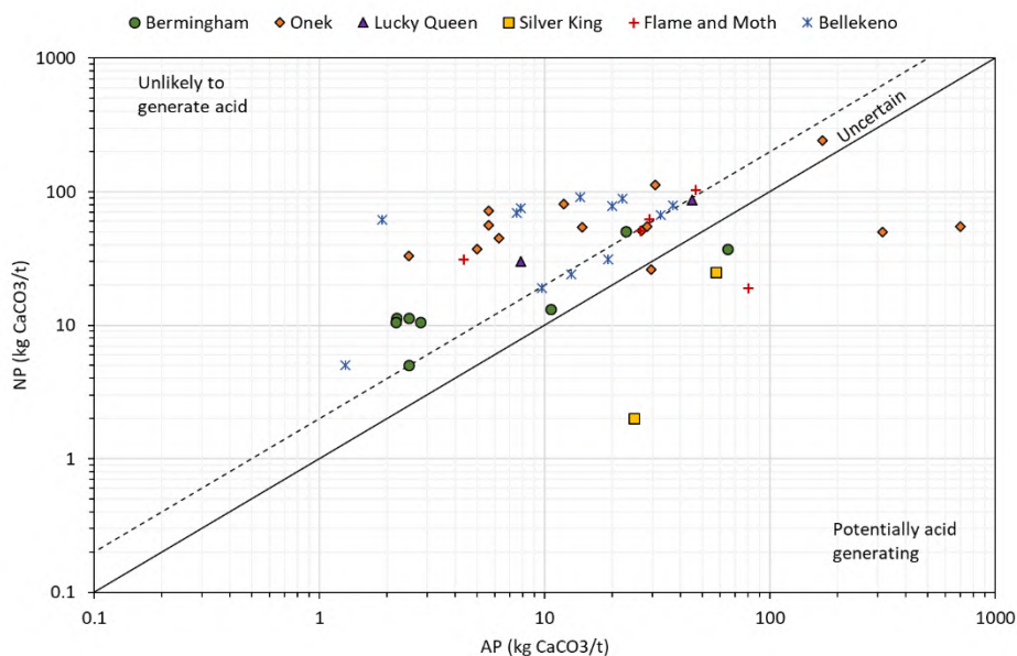
Figure 4-3: Variability in NP and AP of GSCH Lithology Waste Rock Samples from KHSD Deposits
