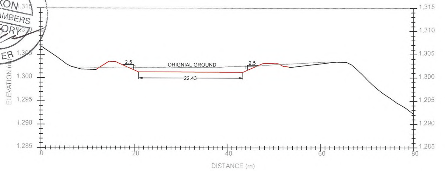
SECTION B
