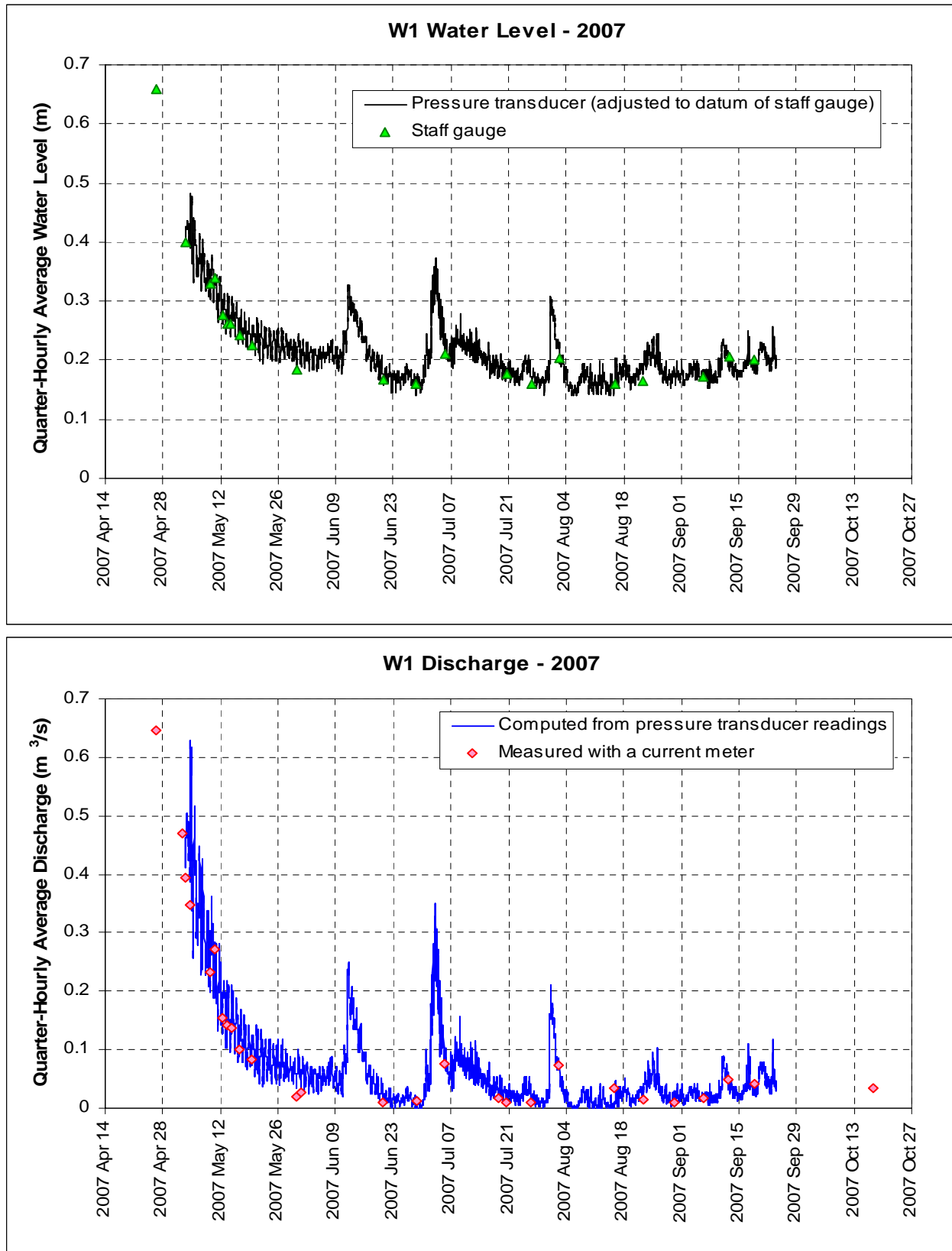
FIGURE MC6-1 - Minto Creek at W1 - Stage and Discharge Records - 2007
