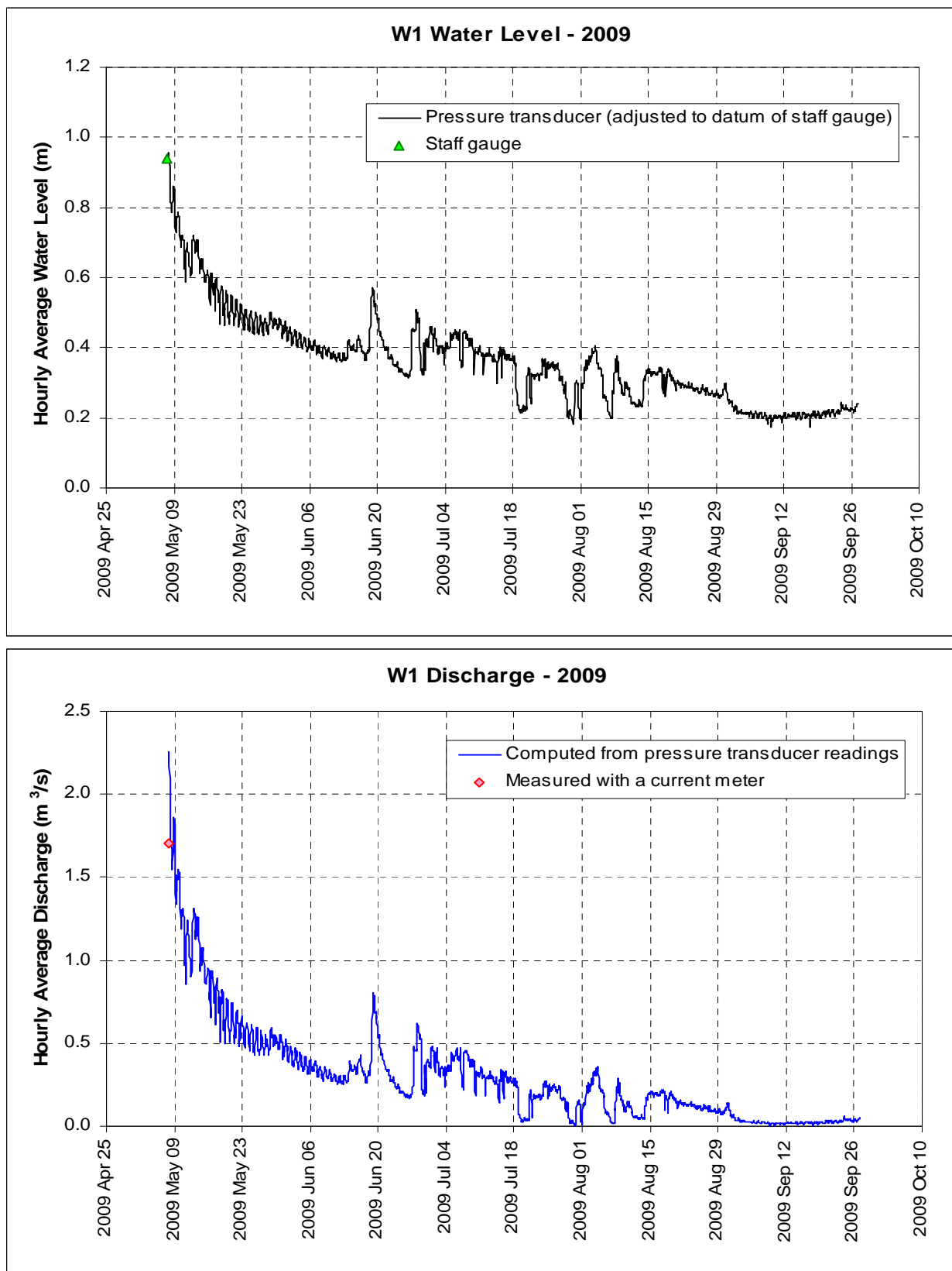
FIGURE MC6-3 - Minto Creek at W1 - Stage and Discharge Records - 2009
