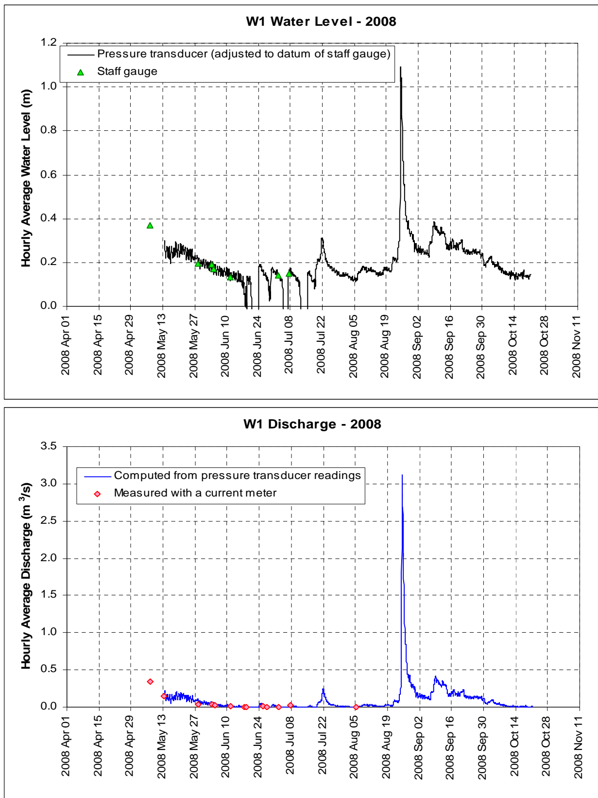
FIGURE MC6-2 - Minto Creek at W1 - Stage and Discharge Records - 2008
