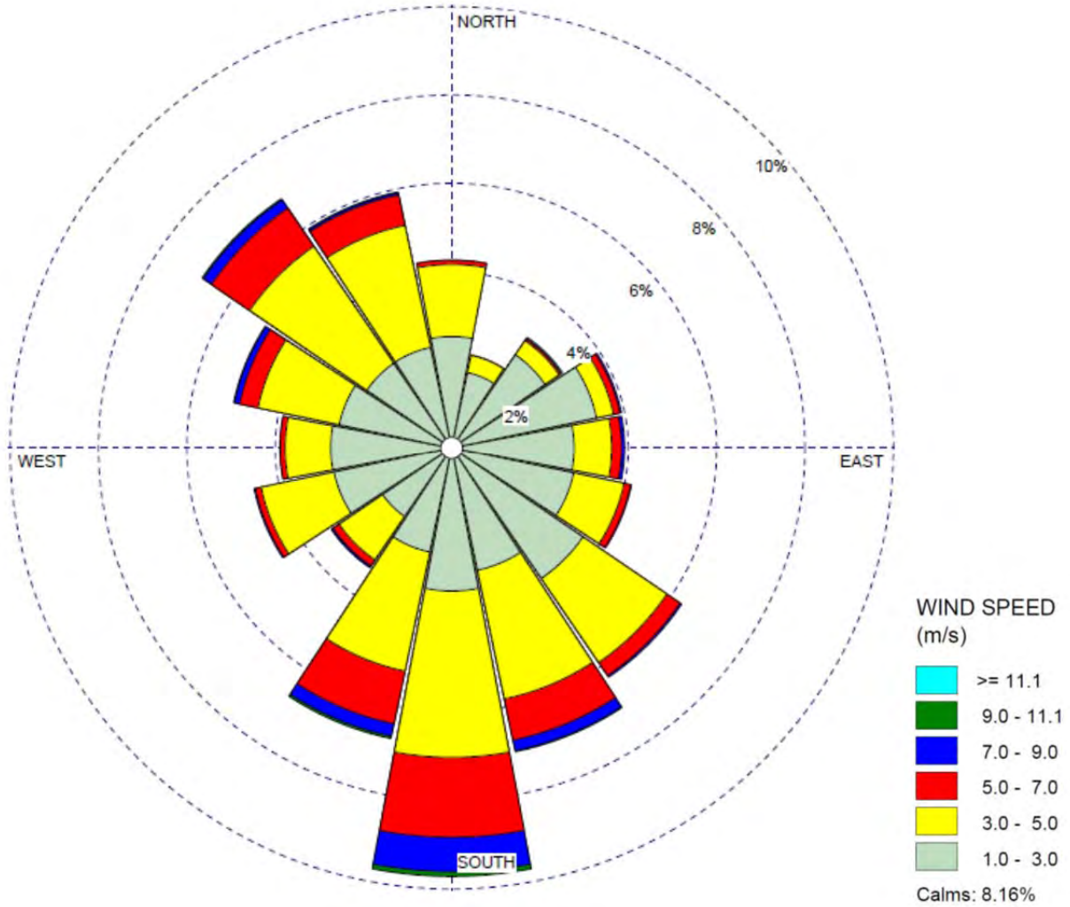
Figure 3-10: Minto HOB0 Meteorological Station Wind Plot, September 2005–April 2010.
