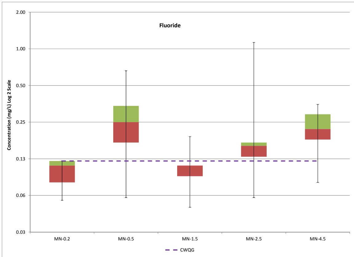
Figure 4-31: Fluoride Boxplots.
