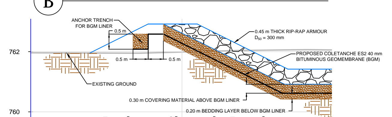
1 Ditch 400 Channel - Detail
