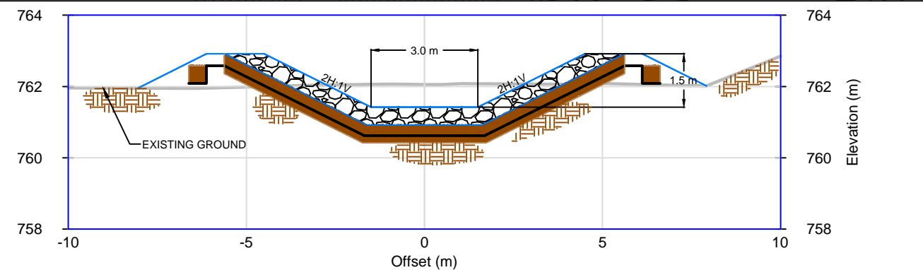
B DITCH 400 TYPICAL SECTION
