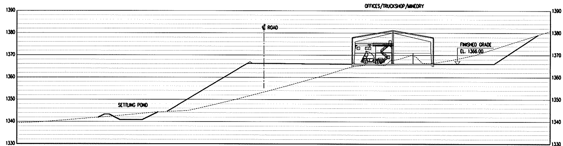
SECTION C 006
