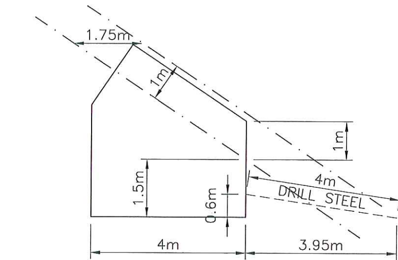
SIDE SLASH MIN ORE THICKNESS
