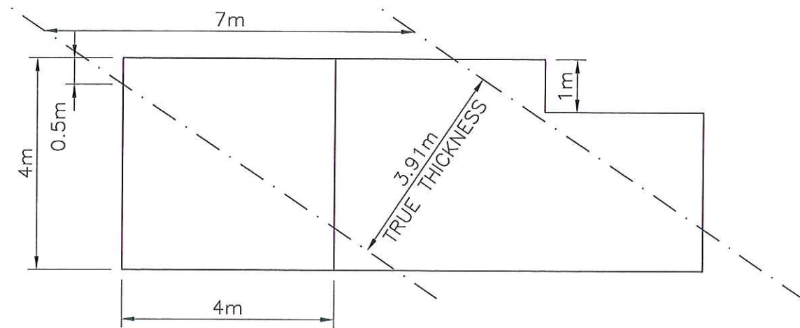
ROOM PILLAR MIN ORE THICKNESS
