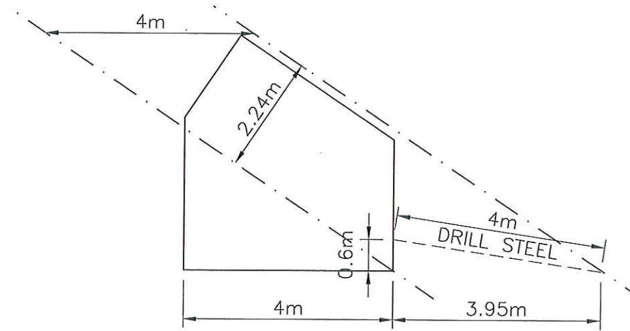
SIDE SLASH MAX ORE THICKNESS
