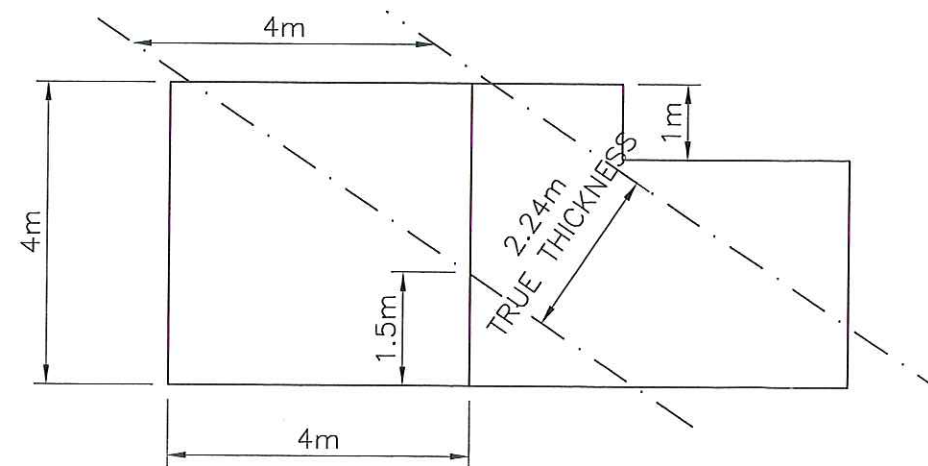
RETREAT PANEL MIN ORE THICKNESS
