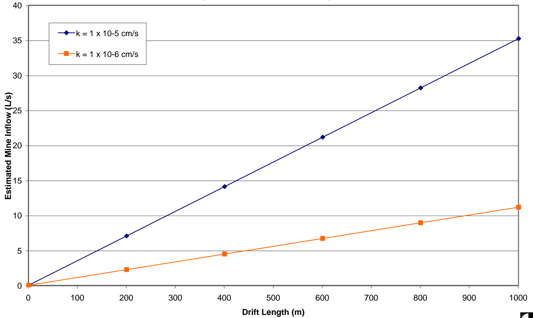
Figure 6.4-10: Mine Inflow Estimate versus Drift Length (After Goodman et al., 1965)
