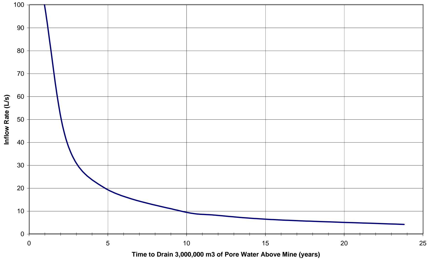
Figure 6.4-11: Years to Drain Pore Water Above Mine vs Inflow Rate
