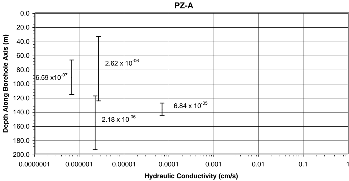
Figure 6.4-3: Hydraulic Conductivity versus Depth (Plotted over Test Interval)
