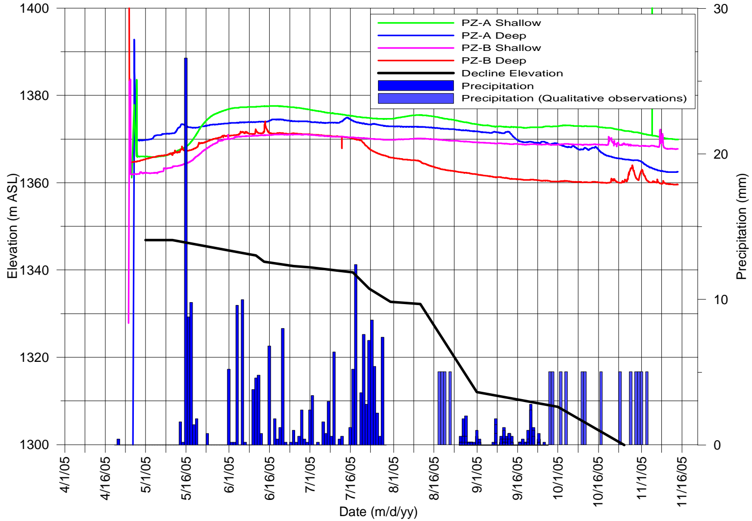
Figure 6.4-4: Measured Potentiometric Groundwater Elevations in Mine Area Piezometers Relative to Decline Advancement
