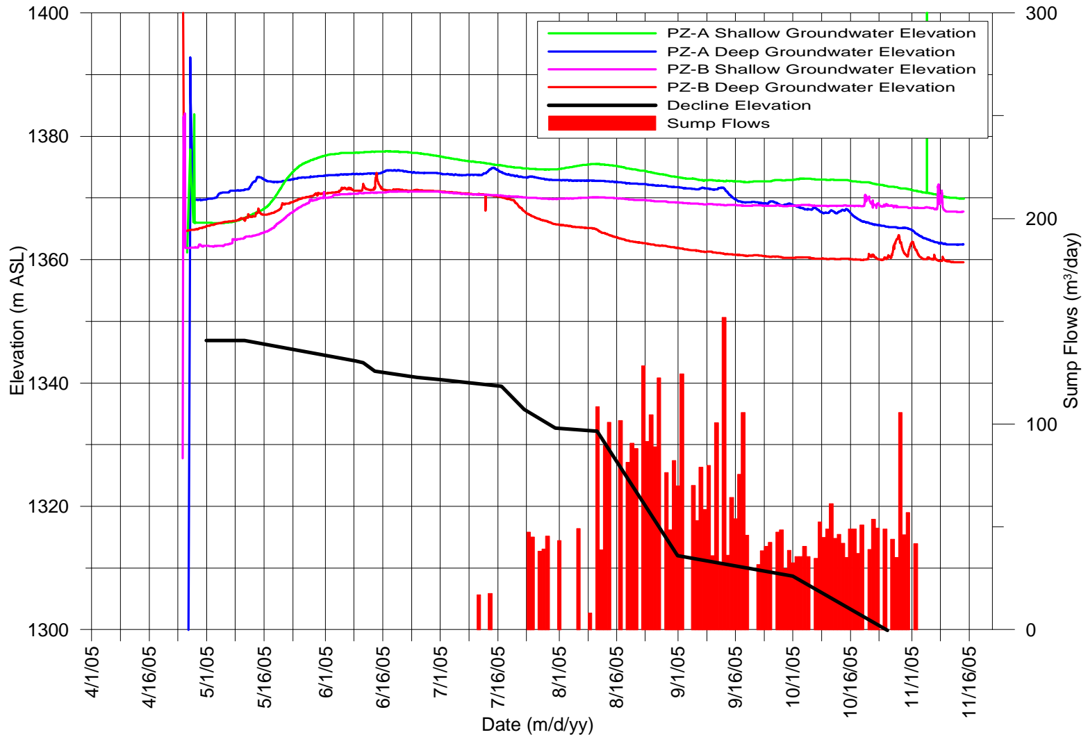
Figure 6.4-5: Measured Potentiometric Groundwater Elevations in Mine Area Piezometers Relative to Decline Advancement
