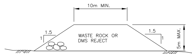
TYPICAL SPLITTER INCREMENTAL DYKE SECTION
