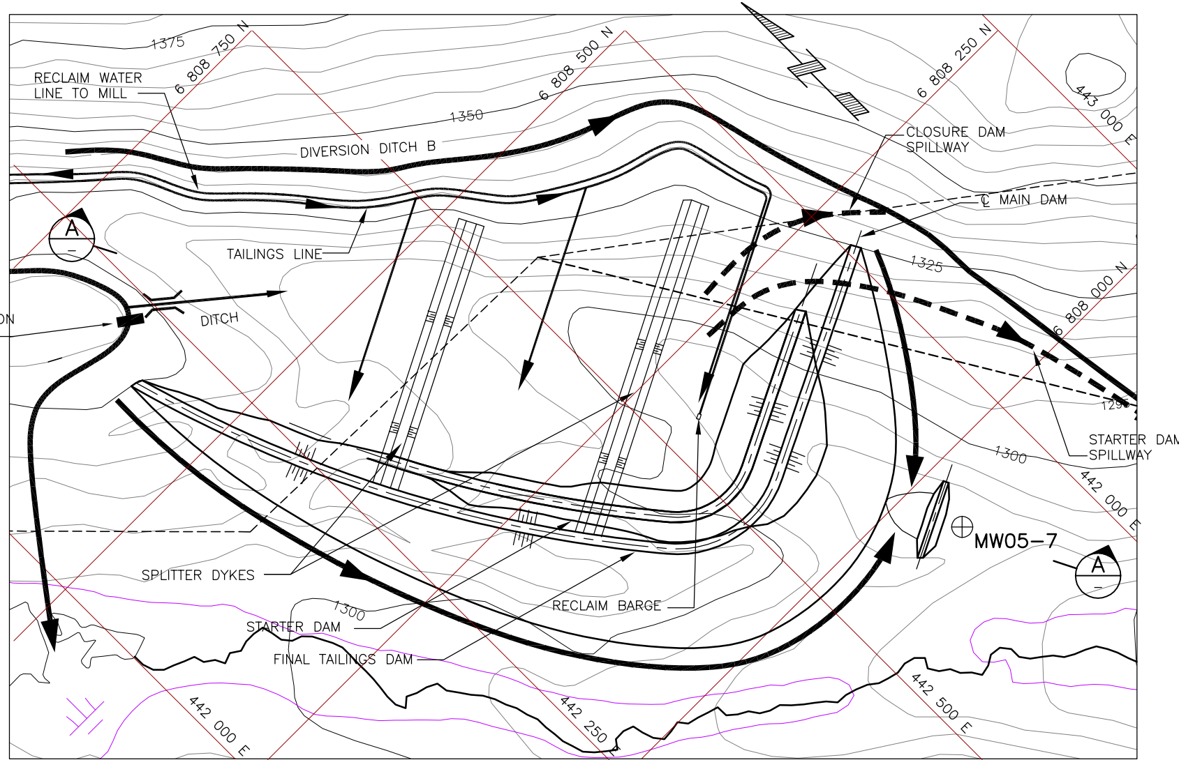
PLAN SCALE A
