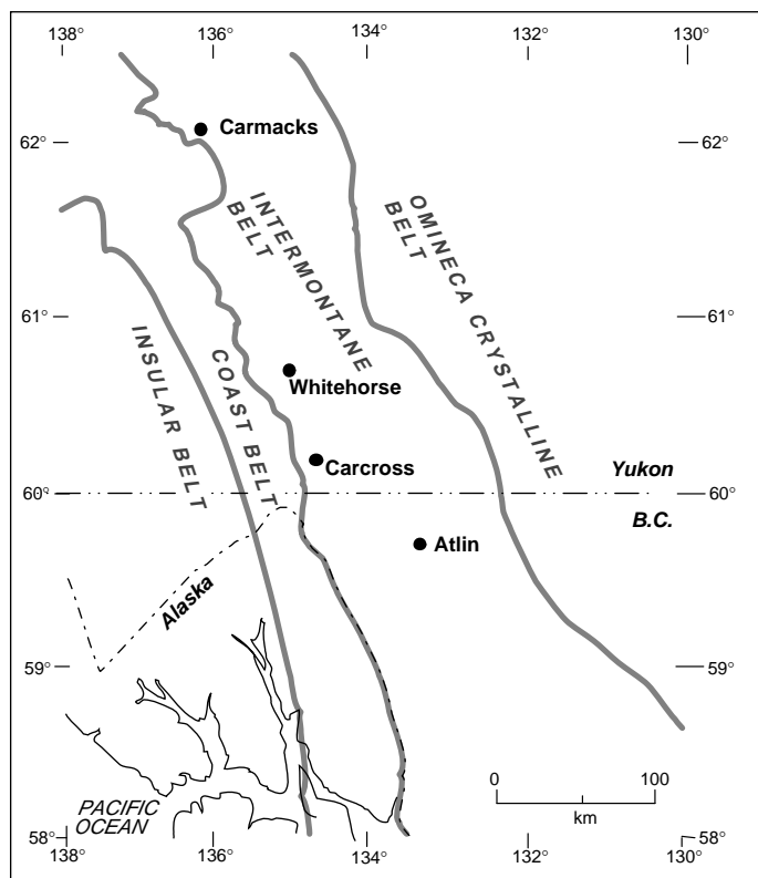
Figure 3. Terrane map.
