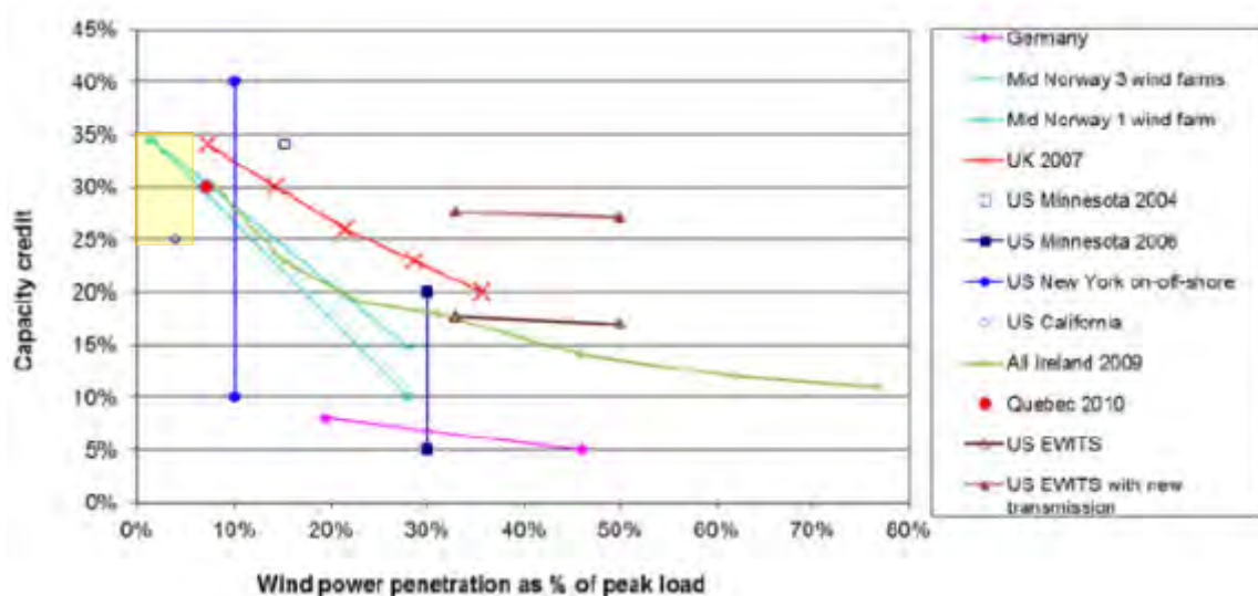
Figure 39 Capacity Credit of Wind Power in Various Parts of the World 11
