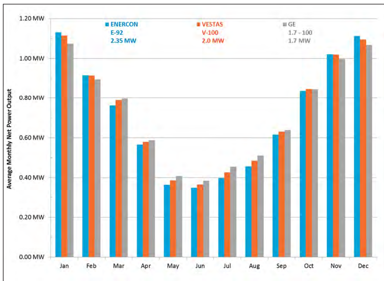
Figure 2 Monthly Generation Profile of a three types of wind turbines at Cyprus Mine Hill
