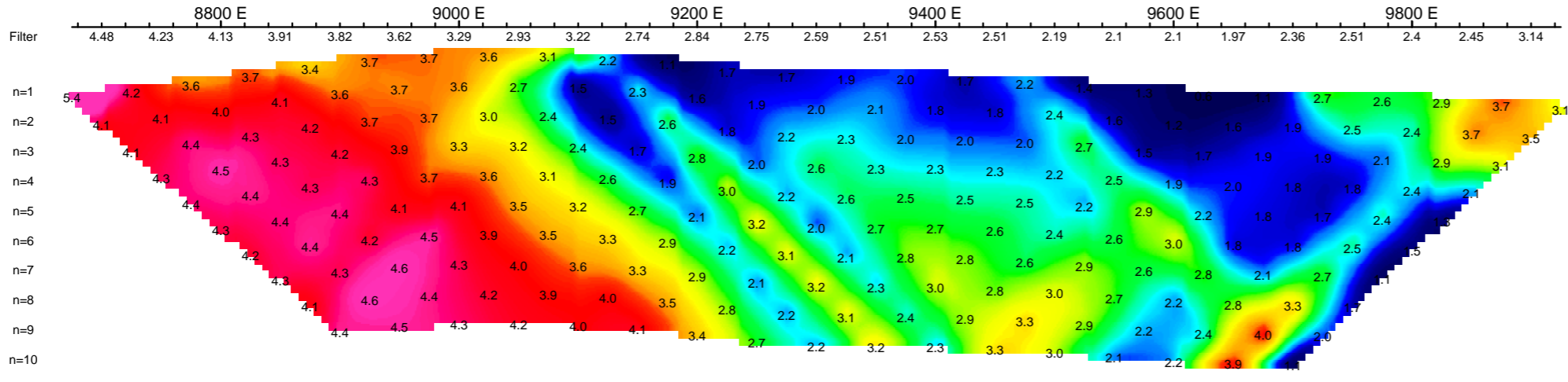
App. Chargeability mV/V
