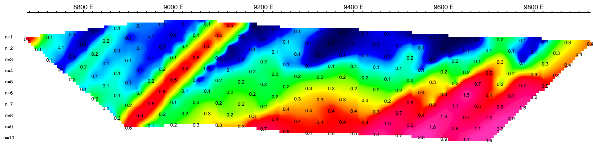
App. Chargeability Err. mV/V
