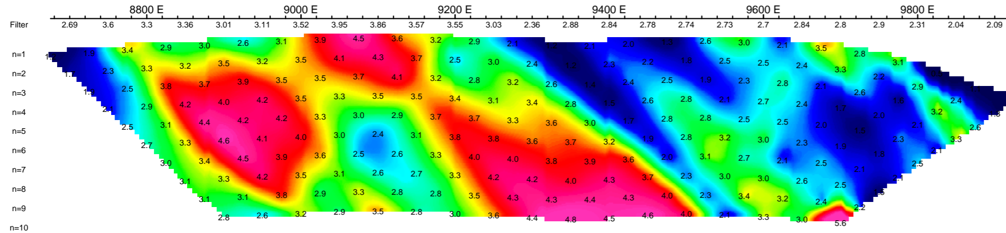
App. Chargeability mV/V
