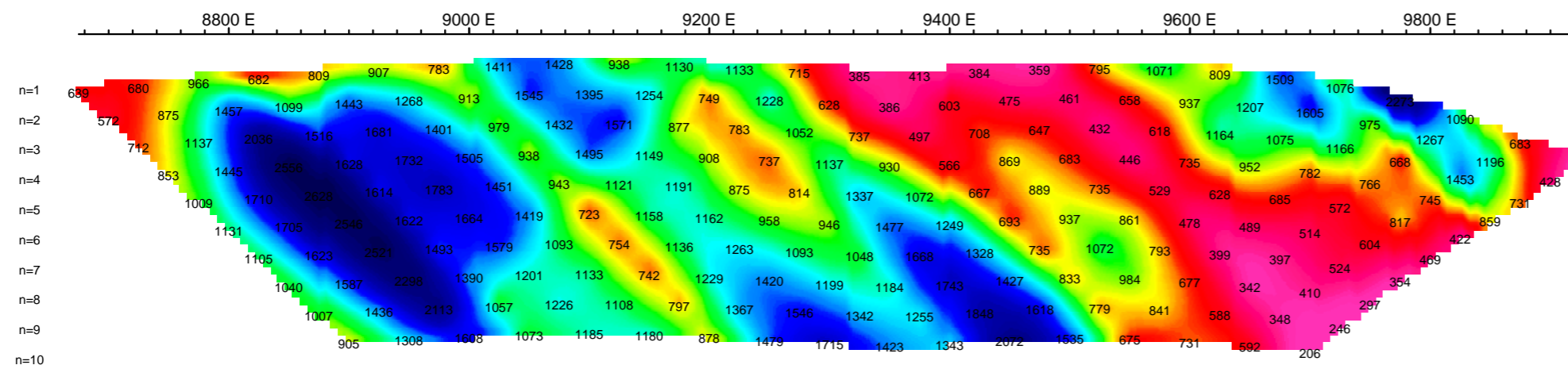
App. Resistivity Ohm*m
