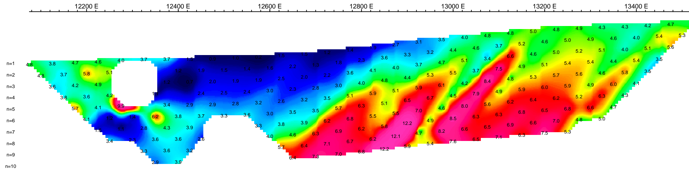
App. Chargeability mV/V
