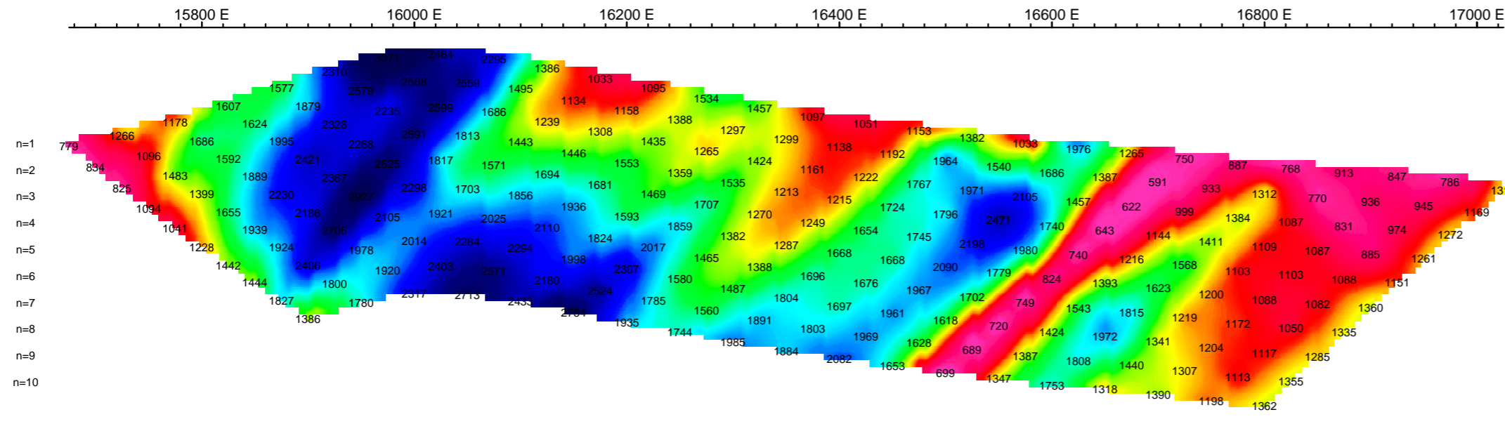
App. Resistivity Ohm*m
