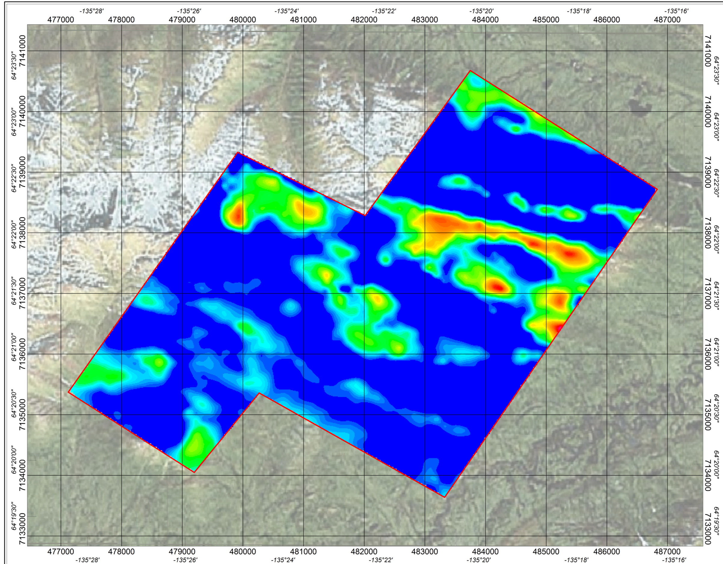
Mean Layer Resistivity ohmm
