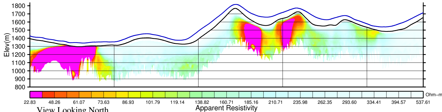
View Looking North Apparent Resistivity
