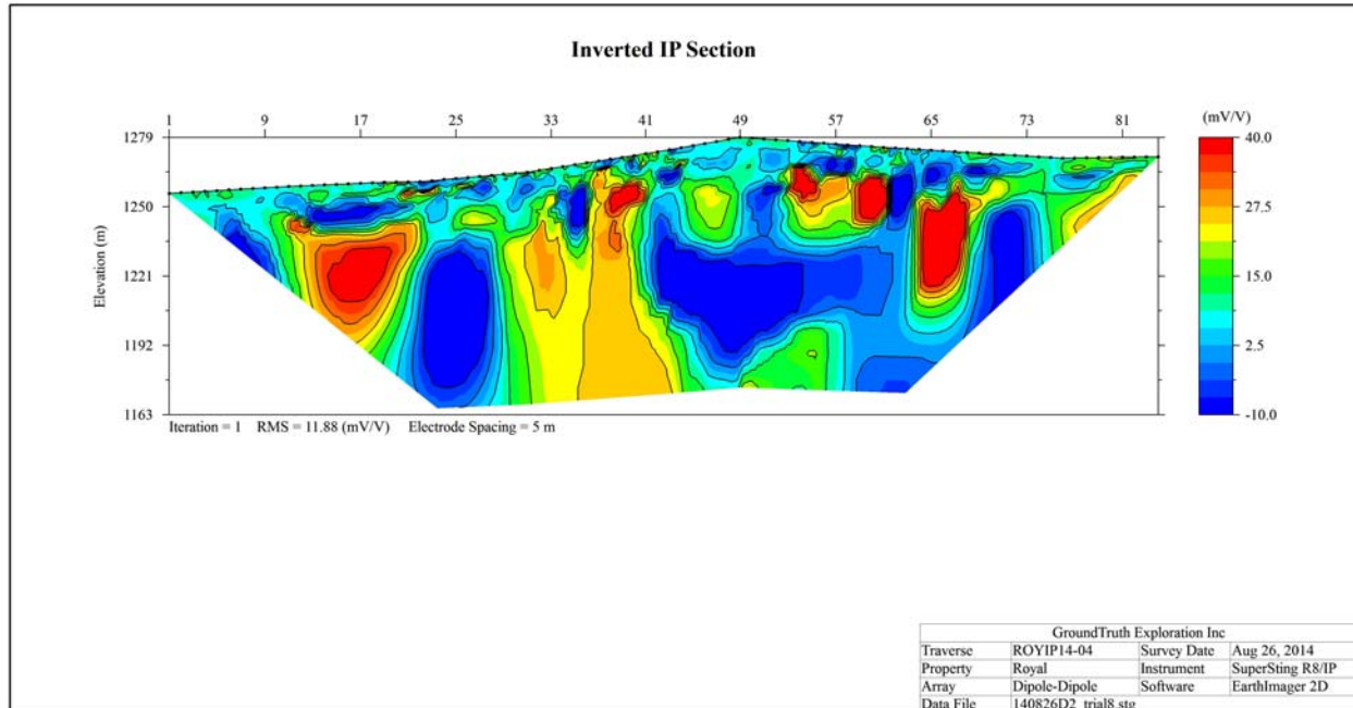
Figure 14: ROYIP14-04 IP
