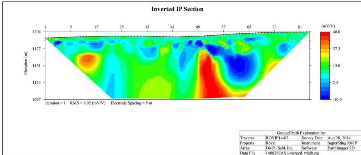
Figure 10: ROYIP14-02 IP
