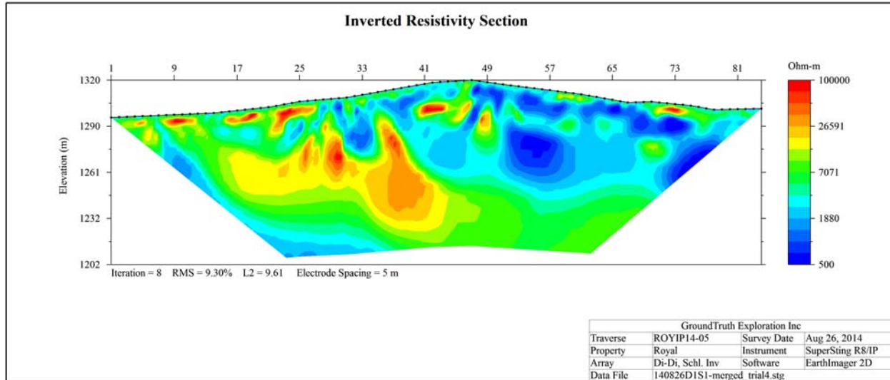
Figure 15: ROYIP14-05 Resistivity
