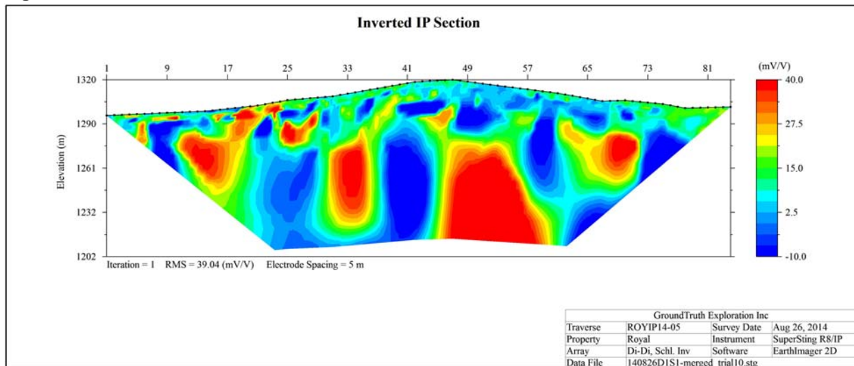
Figure 16: ROYIP14-05 IP
