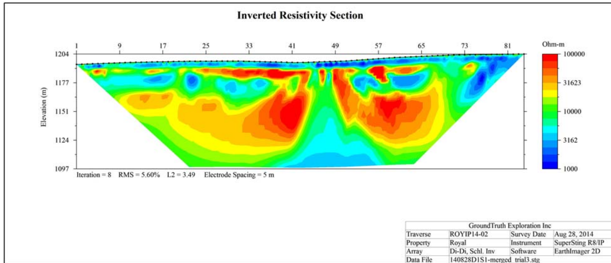
Figure 9: ROYIP14-02 Resistivity
