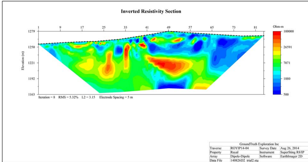
Figure 13: ROYIP14-04 Resistivity
