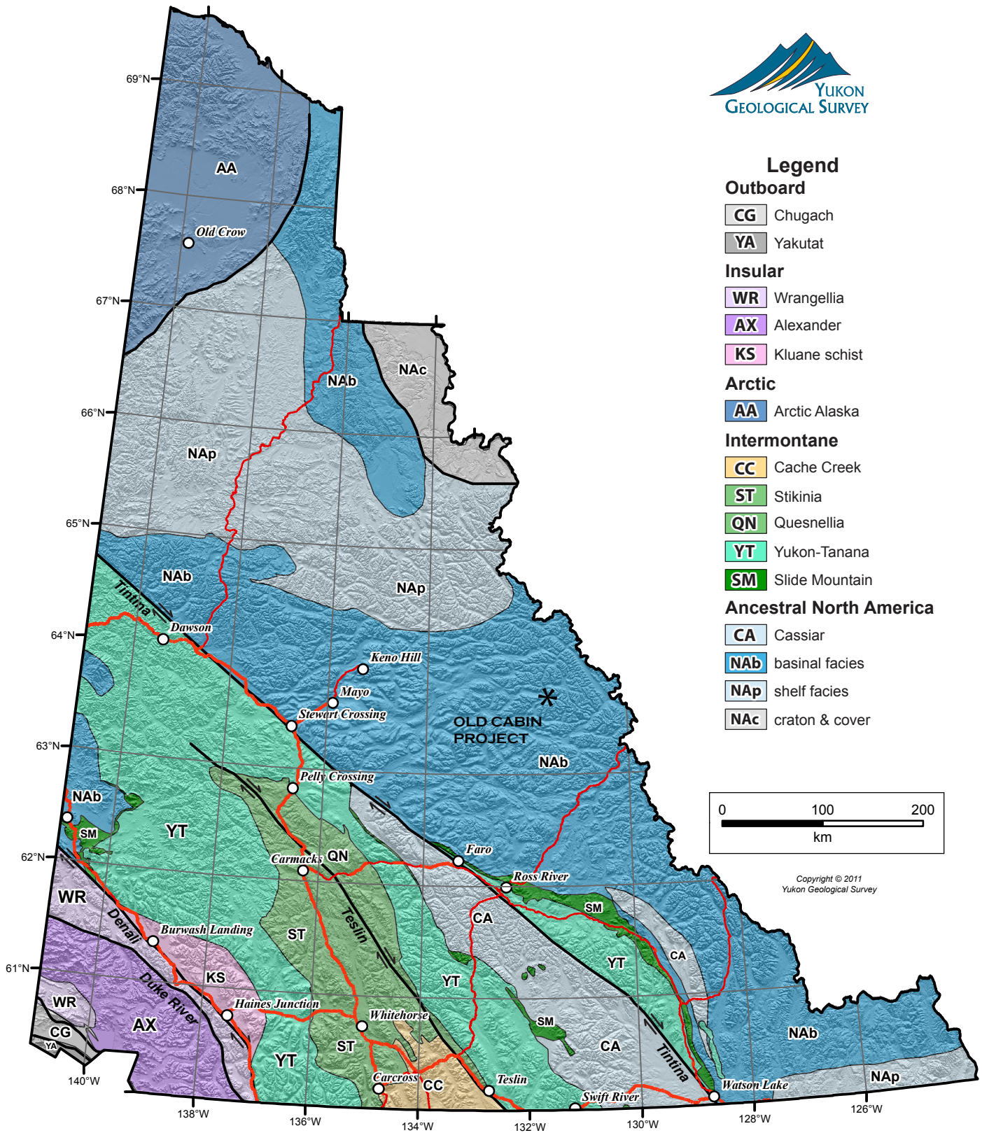
Figure 1. Location and Geological Terranes - Old Cabin Project
