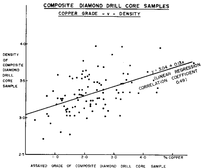
Figure 18. Plot of copper grade against density for composite underground diamond drill core samples. Note the regression line is almost the same as that in figure 32, suggesting that dilution has little influence on density of ore delivered to the mill.
