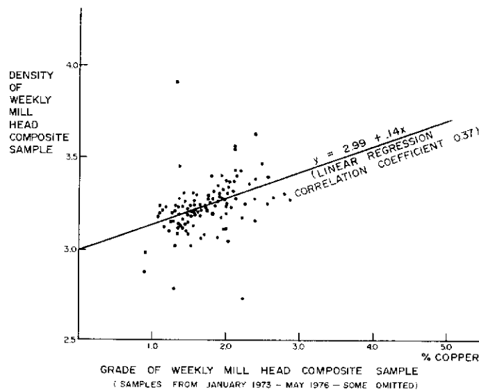
Figure 32. Copper grade plotted against density for weekly mill head composite sample (see also figure 18).
