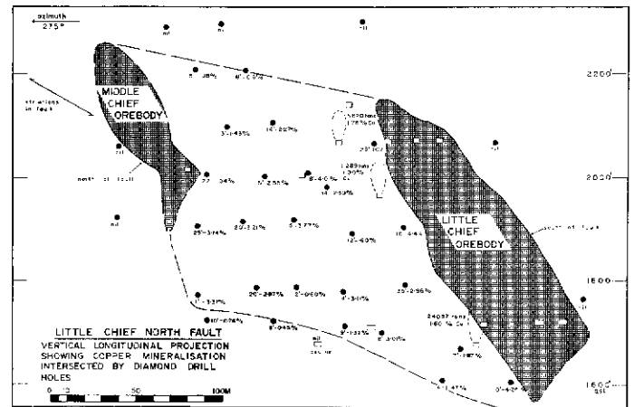
Figure 13. Vertical longitudinal projection along the Little Chief North Fault (see Fig. 14 & 15) showing the location of ore dragged along the fault between Little Chief and Middle Chief ("B" zone). Some of this ore has been mined by block caving and the grade and tonnage extracted is shown. The direction of movement along the fault is indicated by striations, the distribution of ore in the fault and the relative locations of the two offset portions of the orebody.
