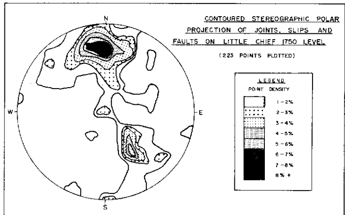
Figure 38. Contoured stereographic polar projection of joints, slips and faults Little Chief underground 1750 level. Two sets of joints dipping approximately 70^{\circ} south and 50^{\circ} north are apparent. The intersection of these two joint sets on the hangingwall side of the stopes induced caving out into the hangingwall rather than slabbing of hangingwall rocks into the stope. The shear zone along the footwall side of the Little Chief underground orebody is not represented in this diagram.
