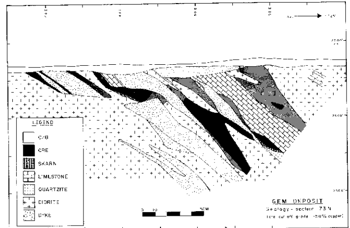
Figure 8. Geological cross-section of the Gem deposit interpreted from surface diamond drilling using a 1.50% copper cut-off grade.
