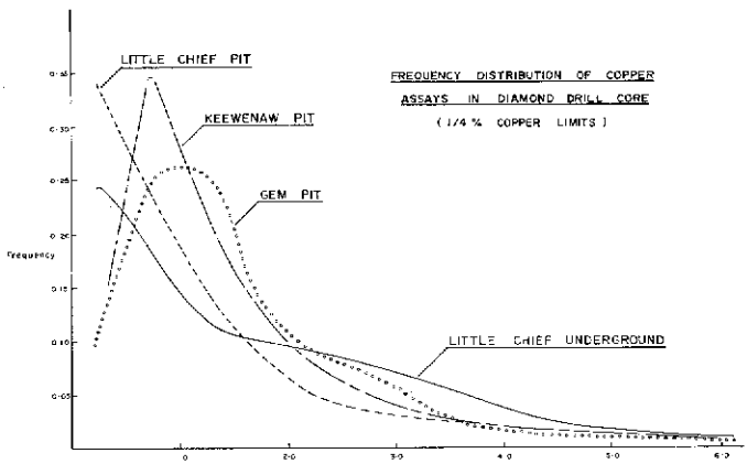
Figure 33. Frequency distributions of diamond drill core assays from selected open pits and the Little Chief underground mine. Curves are skewed positively. The Gem pit looks most attractive on this basis but mining difficulties offset this.
