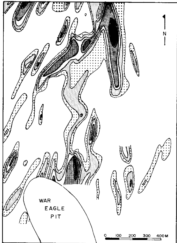
Figure 26. Anomalous train shaped copper dispersion patterns in overburden at Pueblo. These patterns, which may be modified by glacio-fluvial action, indicate the direction of ice movement during the last retreat of Wisconsin ice.
