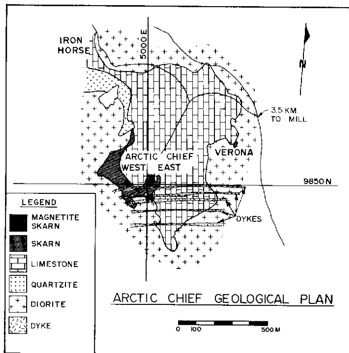
Figure 21. Geological plan of the Arctic Chief pendant.
