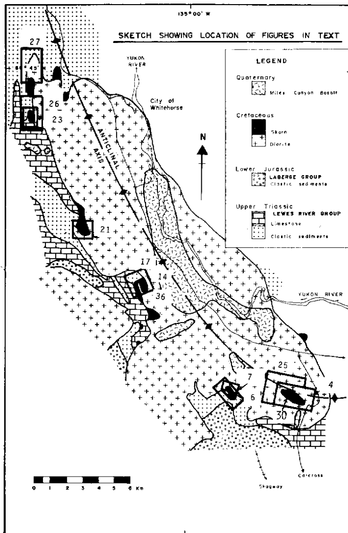
Figure 3. Regional geology of the Whitehorse Copper Belt showing the location of text figures.
