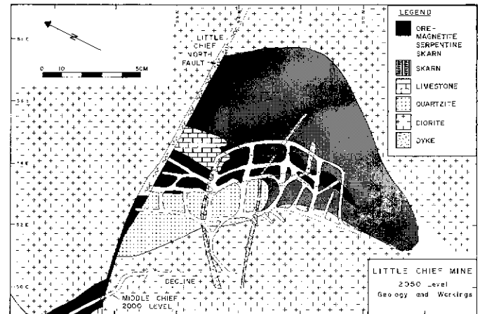
Figure 14. Geological plan of the Little Chief 2050 level showing mine workings and the relationship of "quartzite", ore, skarn and hangingwall limestone in the Little Chief flank pendant. The Middle Chief "B" zone lies north of the Little Chief North Fault. Ore dragged along the fault is also shown.
