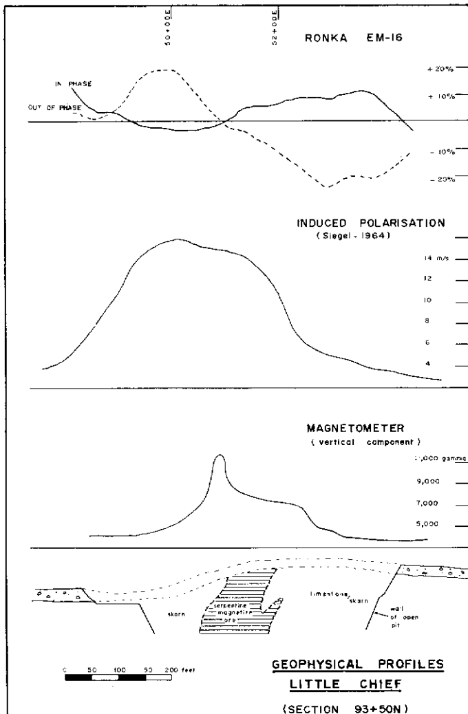
Figure 16. Geophysical profiles across the Little Chief open pit. The magnetometer and IP responses are characteristic. The E.M. - 16 profile is weakly anomalous.
