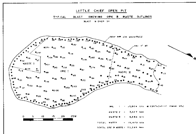
Figure 36. Typical open pit blasthole layout (the Little Chief 2425 - 01 blast) showing the spacing of drill holes, and preshear holes around the pit wall. Areas of waste and ore planimetered converted to waste and ore tonnage blasted are also shown.
