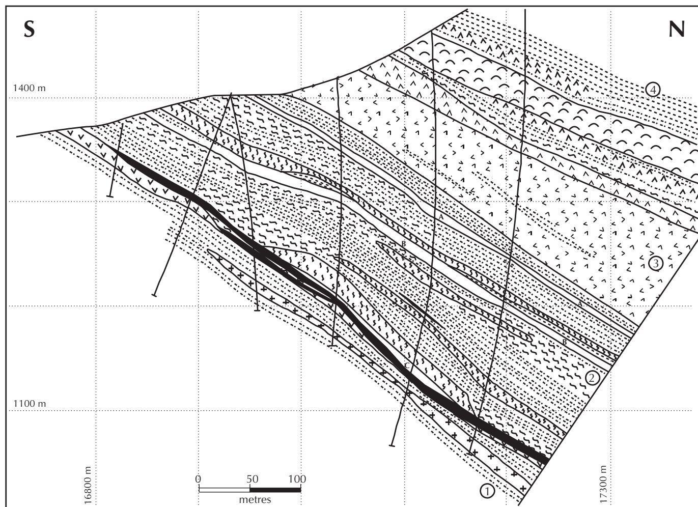
Figure 6. Geological cross-section 16250E through the Lynx zone of the Wolverine deposit. The location of this cross-section is shown on Figure 9. Constructed from detailed geological mapping of drill core, drill logs and cross-sections supplied by Expatriate Resources Limited. Coordinates (in metres) are from the property grid (Fig. 9). Unit numbers and patterns shown in Figure 5.
