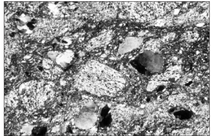
Figure 6. Quartz and sericite replacing elongate feldspar grains in felsic metavolcanic unit. Field of view = 7.2 mm.
