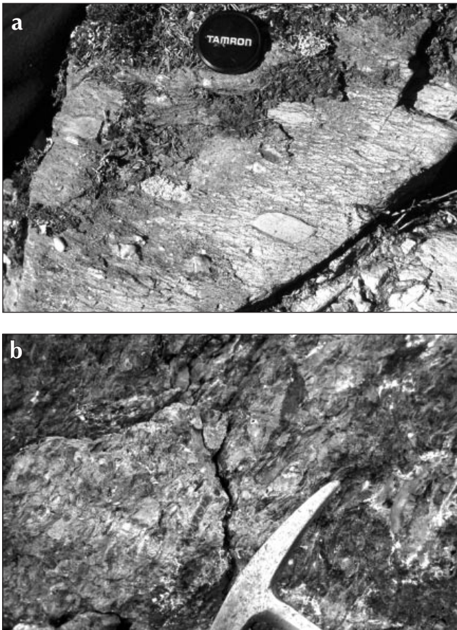
Figure 13. Unit mPcgl: (a) polymictic conglomerate in exposure along Campbell Highway; (b) limestone and chert clasts in an isolated exposure of polymictic conglomerate about 5 km south of King Arctic jade mine.
