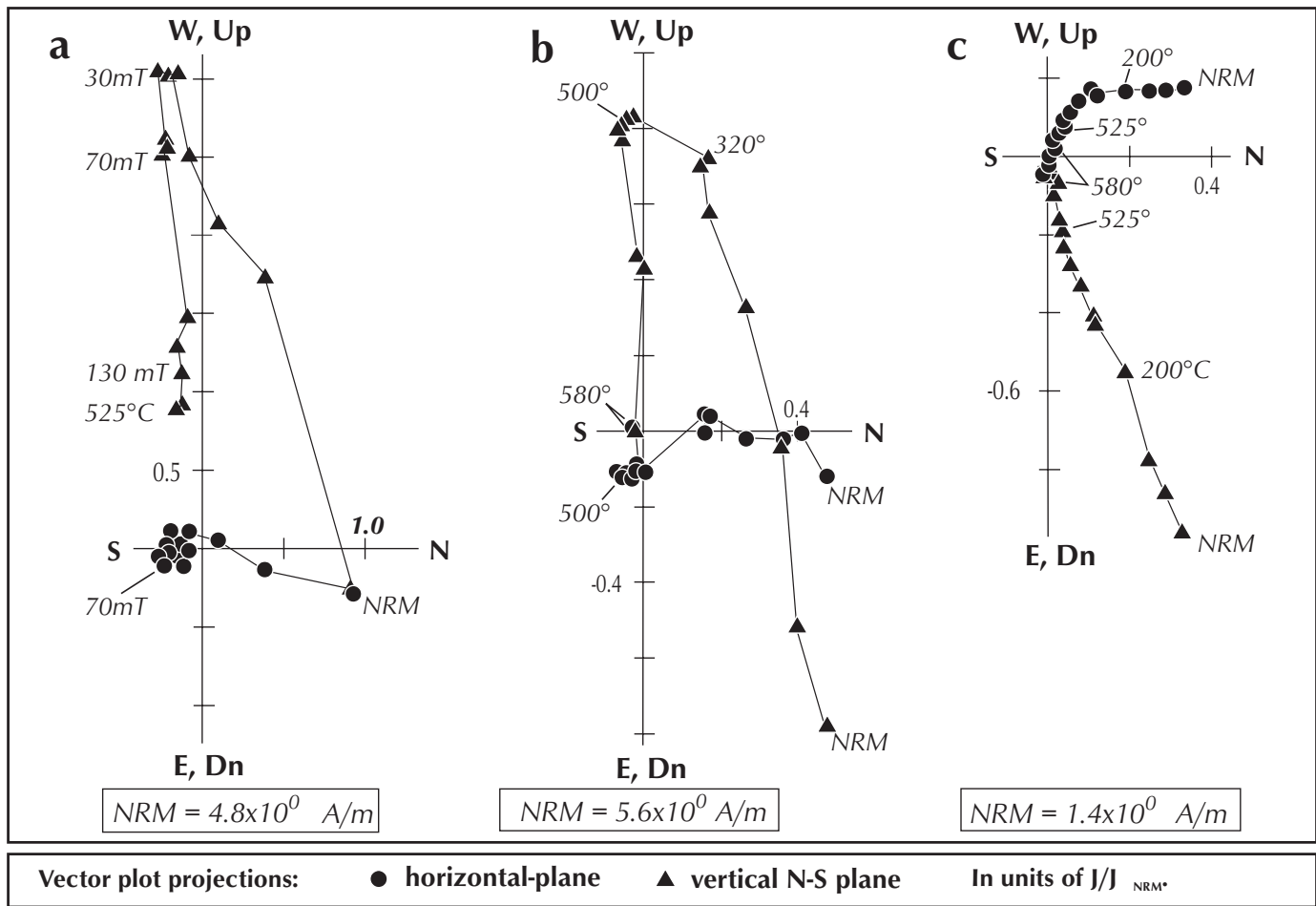
Figure 5. Stepwise demagnetization vector plots for reversed ChRM in specimens from: (a) site 6, (b) site 4, and (c) for a normal ChRM at site 9.
