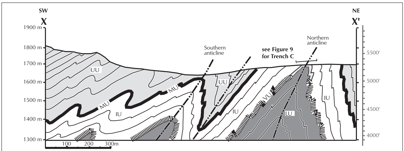
Figure 5b. Summary vertical section across the TBMB area, based on the demonstration of the Southern and Northern anticlines, with an inferred intervening syncline. Two other kilometre-scale F_2 folds have been interpreted along the normal limb of the Southern anticline. F_1 folds have been omitted, basically for a reason of scale, but they have been noticed in several outcrops. Details in text.
