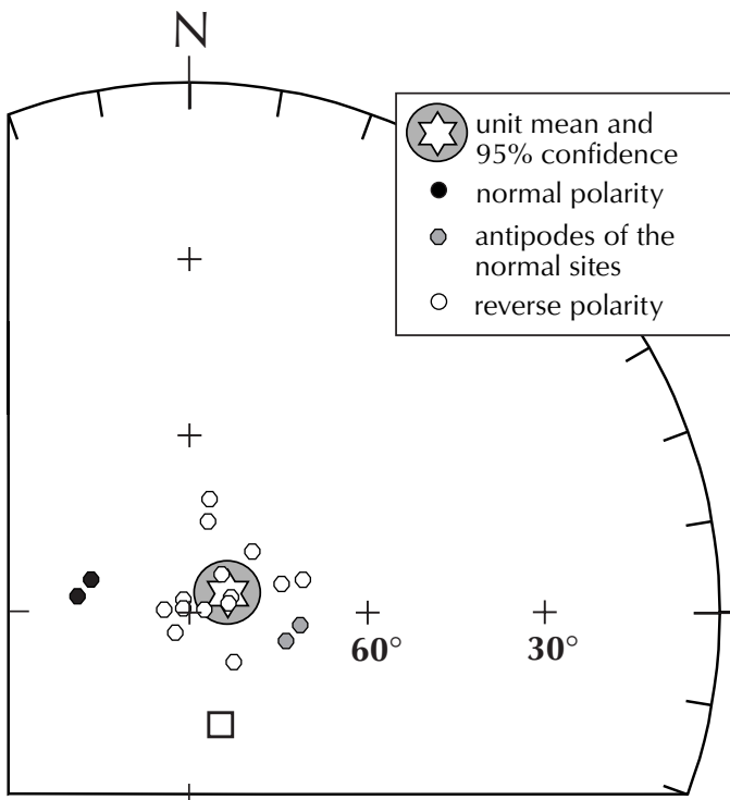
Figure 6. Equal area stereoplots of site and unit mean ChRM directions for the Seymour Creek stock (16 sites). The open square marks the mean direction reported for the Carmacks Group volcanic rocks by Wynne et al. (1998).
