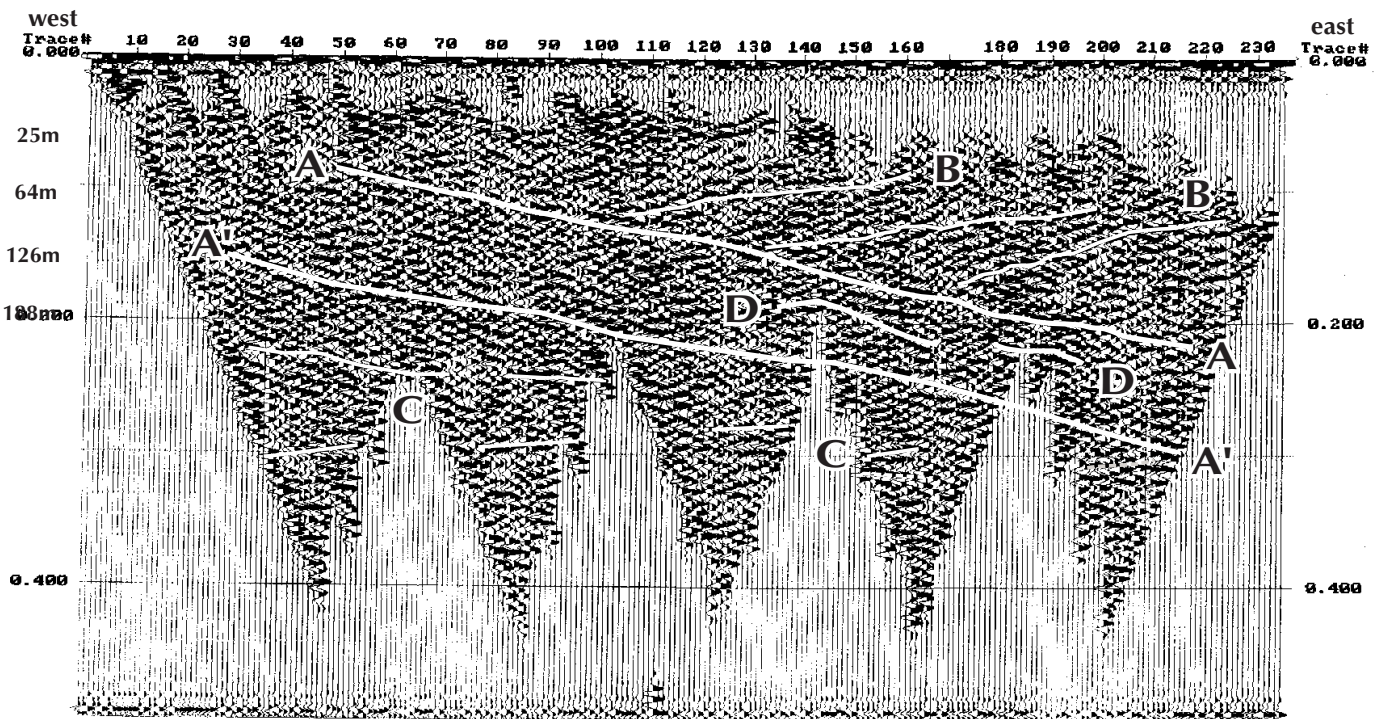
Figure 2. Seismic profile generated from survey undertaken along the high-voltage transmission line south of Riverdale with highlighted reflectors. Vertical scale of two-way travel-time in milliseconds. Metre-scale approximate as it is model dependent. Numbers on horizontal scale are geophone sites. Total horizontal section is approximately 560 m. Interpretations of results are in the text.
