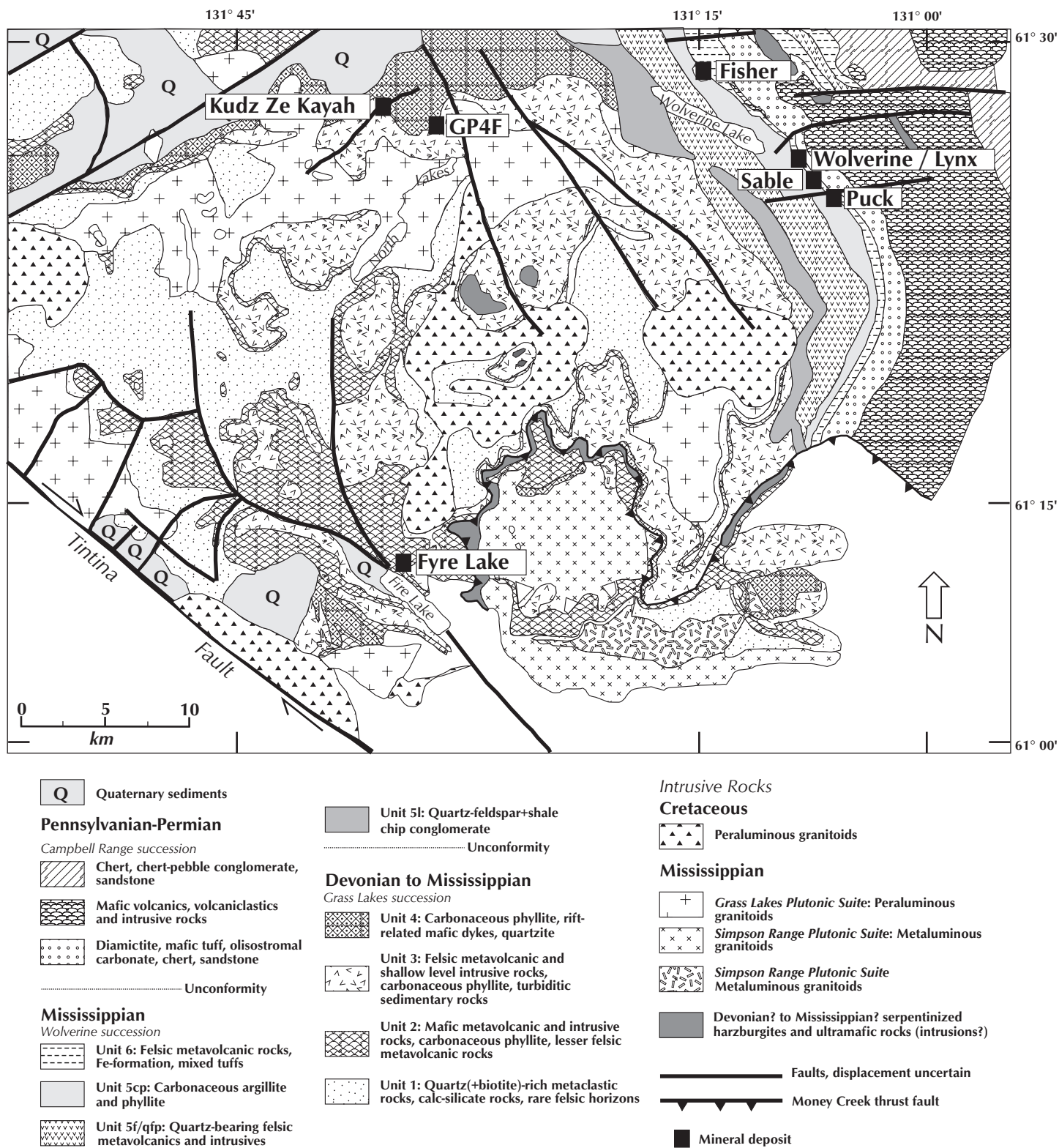
Figure 2. Geological map of the Finlayson Lake region modified from Murphy (1998) and Piercey et al. (1999) with locations of different zones of the Wolverine VHMS deposit and other VHMS deposits of the Finlayson Lake district.
