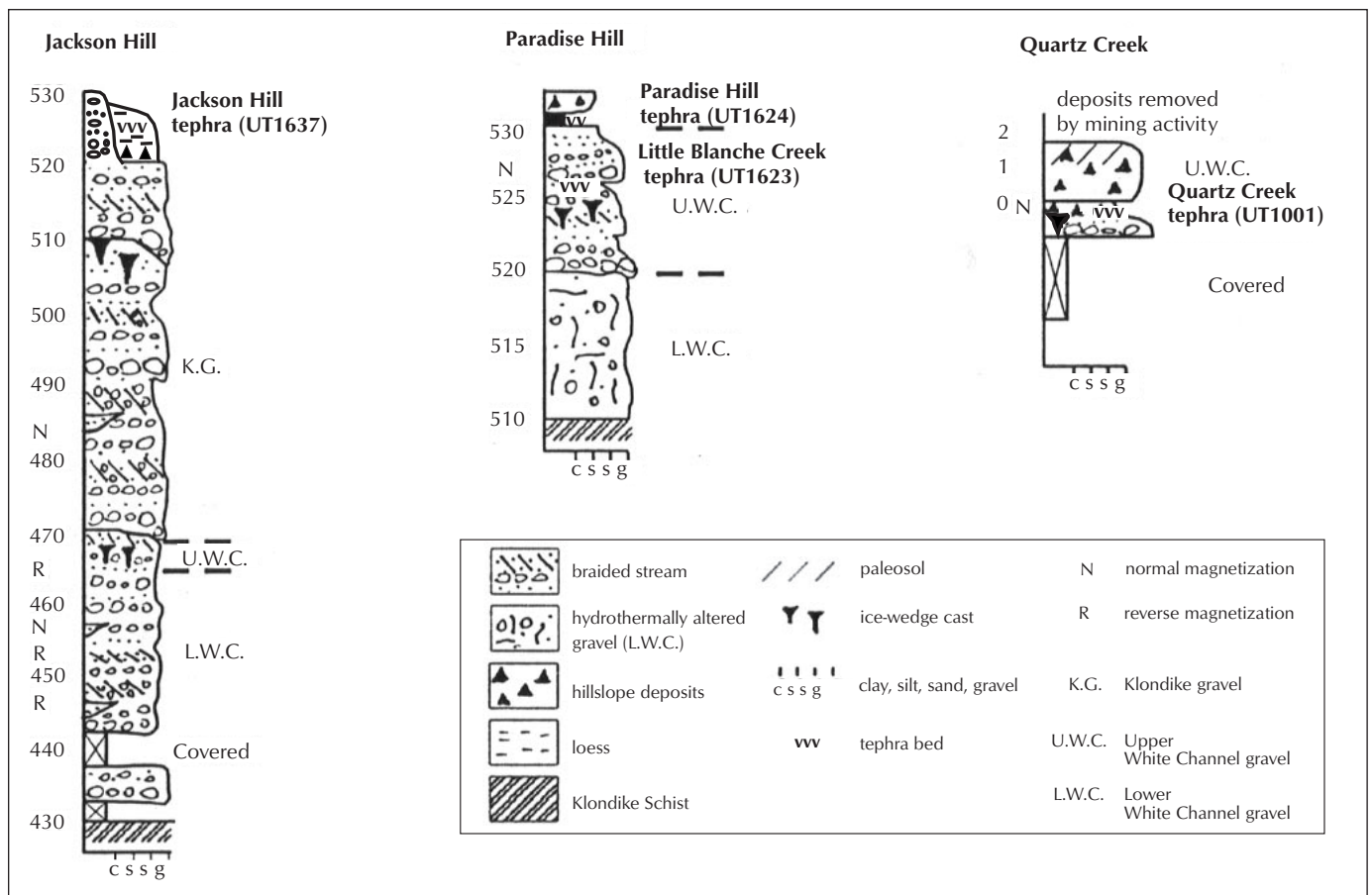
Figure 2. The lithostratigraphic setting of tephra beds at Jackson Hill, Paradise Hill and Quartz Creek sites. Elevation in metres is given for the first two localities, but only the thickness is given for the Quartz Creek site.
