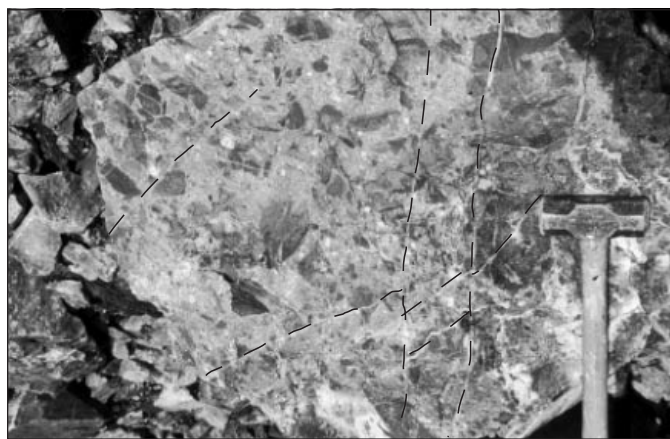
Figure 4. Veined intrusive breccia from the Saddle stock. The dark fragments are mostly phyllite and the matrix is porphyritic quartz monzonite. The intrusive breccia is cut by mineralized quartz + potassium feldspar veins in two distinct orientations highlighted by dashed lines.
