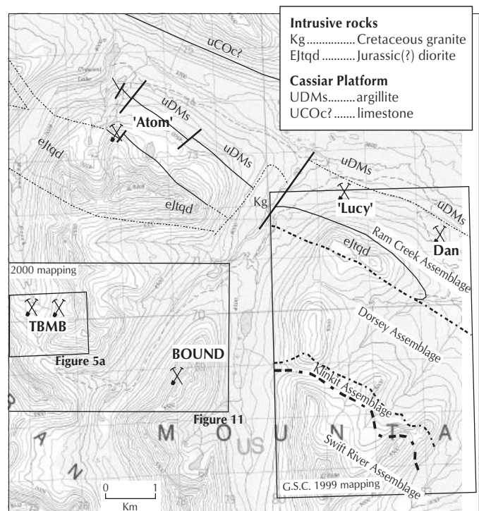
Figure 3. Topographic map (NTS 105B/3) of the upper Swift River area indicating the spatial relationship of showings mentioned in the text. Some contacts are shown from regional mapping by Stevens and Harms (2000); faults are heavy dashed lines.
