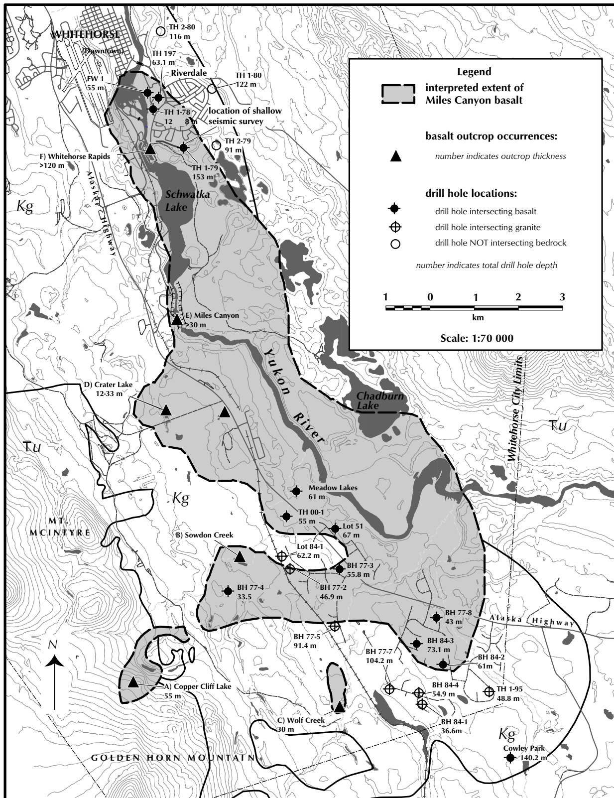
Figure 1. Interpreted extent of Miles Canyon basalt in the Whitehorse area, with localities of drill holes and outcrops indicated in the Tables. Distribution of basalt was identified through compilation of outcrop localities, reported basalt intersections in drill hole data, interpretation of regional aeromagnetic data, and a reflected seismic survey. Kg = Cretaceous granite; Tu = Triassic Whitehorse Trough sedimentary rocks.
