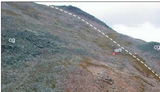
Figure 7. Looking northeast towards the eastern shoulder of the Hy property, where a diamond drill is targeting a north-trending, southwest-dipping structure (dashed line). Note resistant conglomerate (cg). Auriferous soil and rock samples are associated with this structure.
