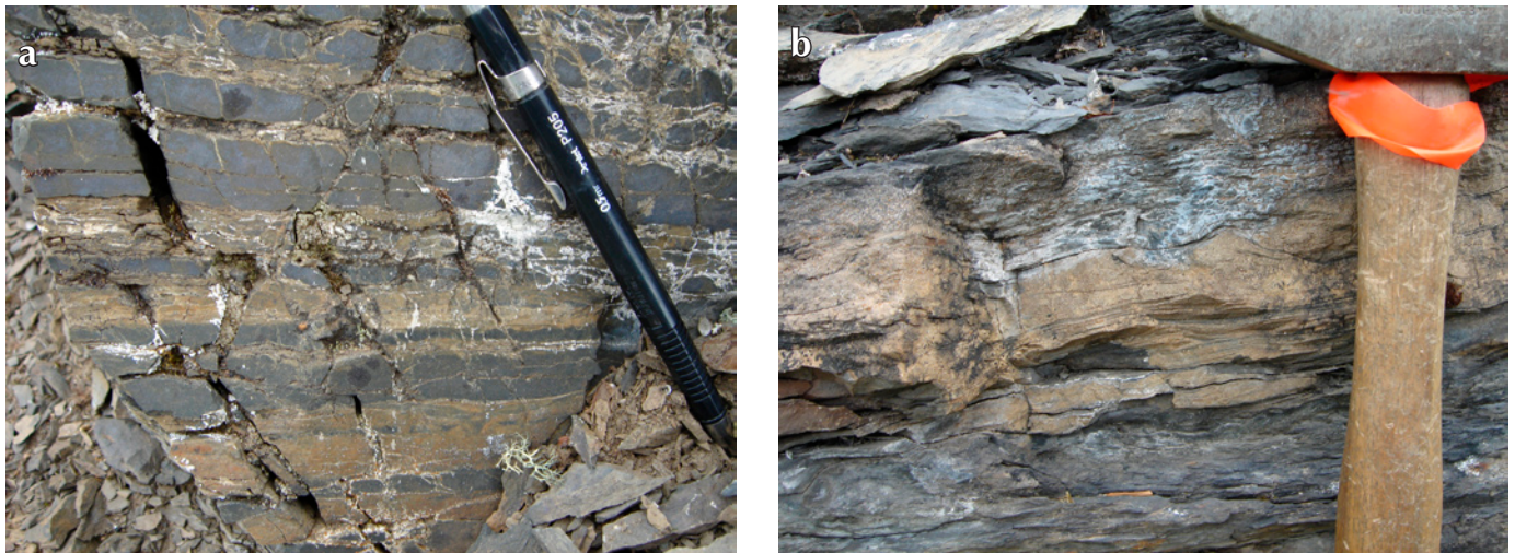
Figure 3. (a) Triassic silty shale with wispy calcareous material, lower member, McNeil Lake area. (b) Triassic silty shale with lenticular silty limestone bodies, middle member, McNeil Lake area. (c) Triassic couplets of limy siltstone and carbonaceous shale, upper member, McNeil Lake area.
