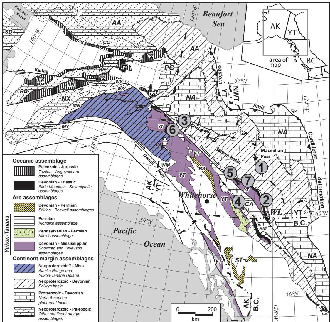
Figure 1. Tectonic assemblage map of the northern Cordillera. Numbered circles indicate Triassic successions of this study. Modified from Colpron et al. (2006).
