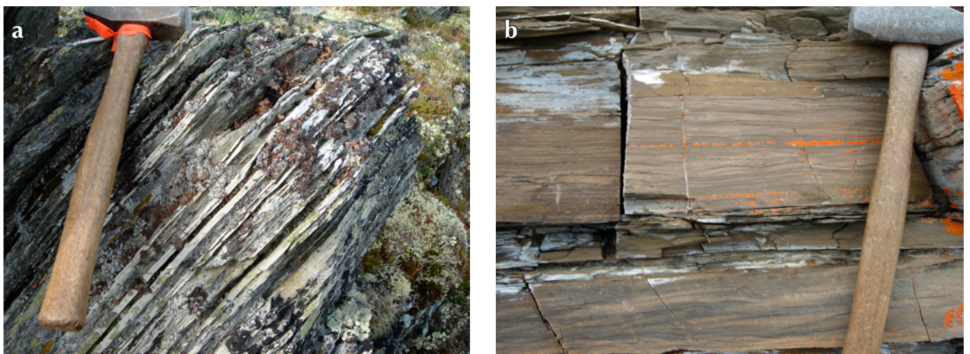
Figure 2. (a) Typical outcrop view of white-green weathering, grey thinly bedded, siliceous Permian shale that underlies Triassic rocks east of Mt. Robert Service, upper Klondike River area. (b) Wavy-laminated calcareous siltstone and sandstone of the lower Triassic succession east of Mt. Robert Service. Detrital mica is pervasive, especially along shale partings.
