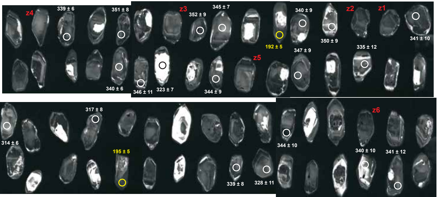
Appendix 6. CL images of zircon from 10-SI-223. Locations of LA-ICPMS spots are shown with dates in Ma. Spot size is 25 microns. Two analyses of Jurassic rims are shown in yellow. Fraction labels for grains dated by CA-TIMS are shown in red; z1-z6 correspond to fractions listed in Appendix 3.
